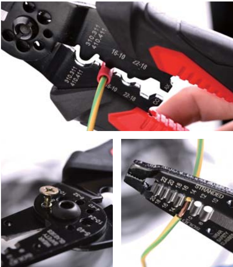
YJTS-2342 Wire Crimper / Stripper
